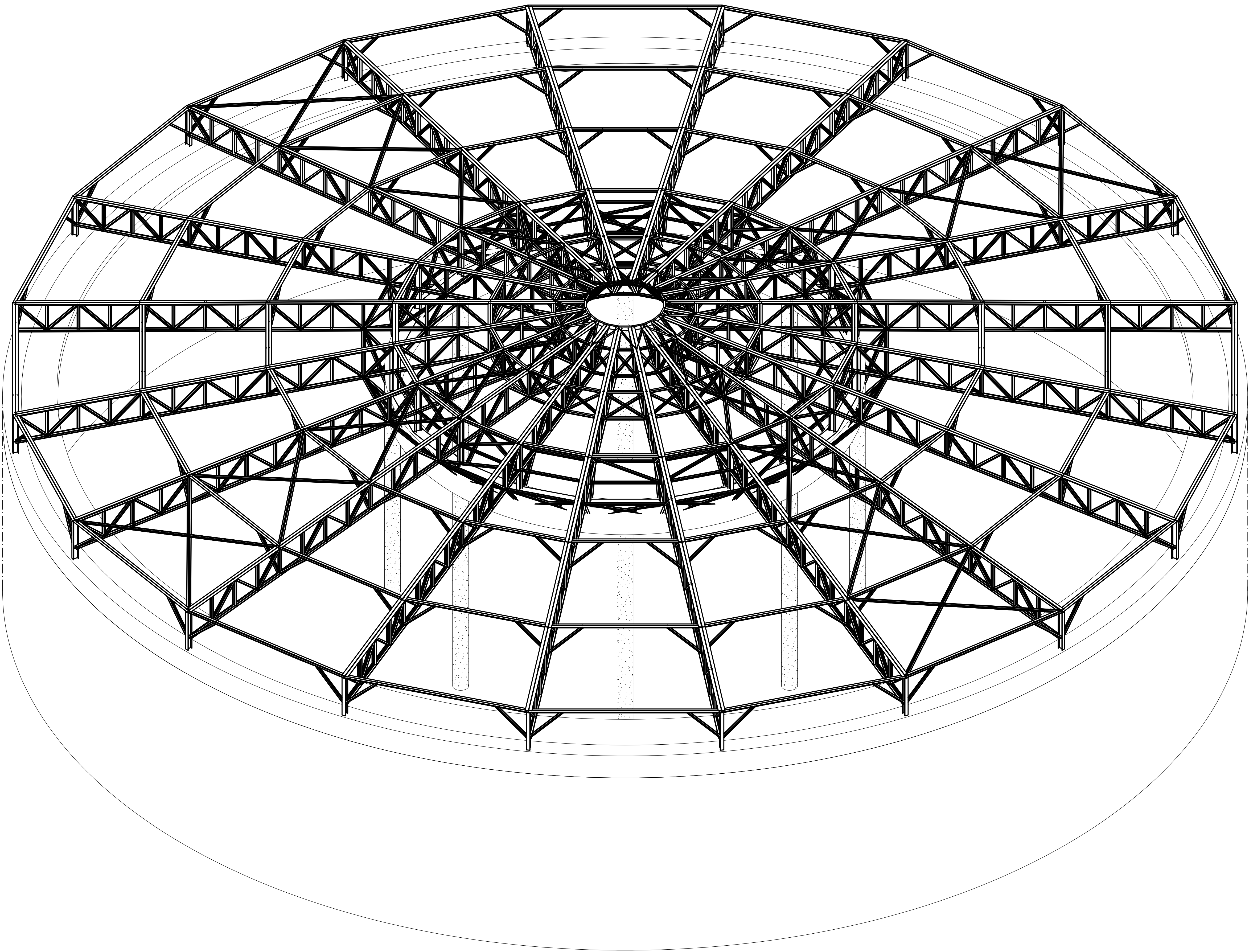
RESERVOIR ISOMETRIC VIEW SCALE 1:75
