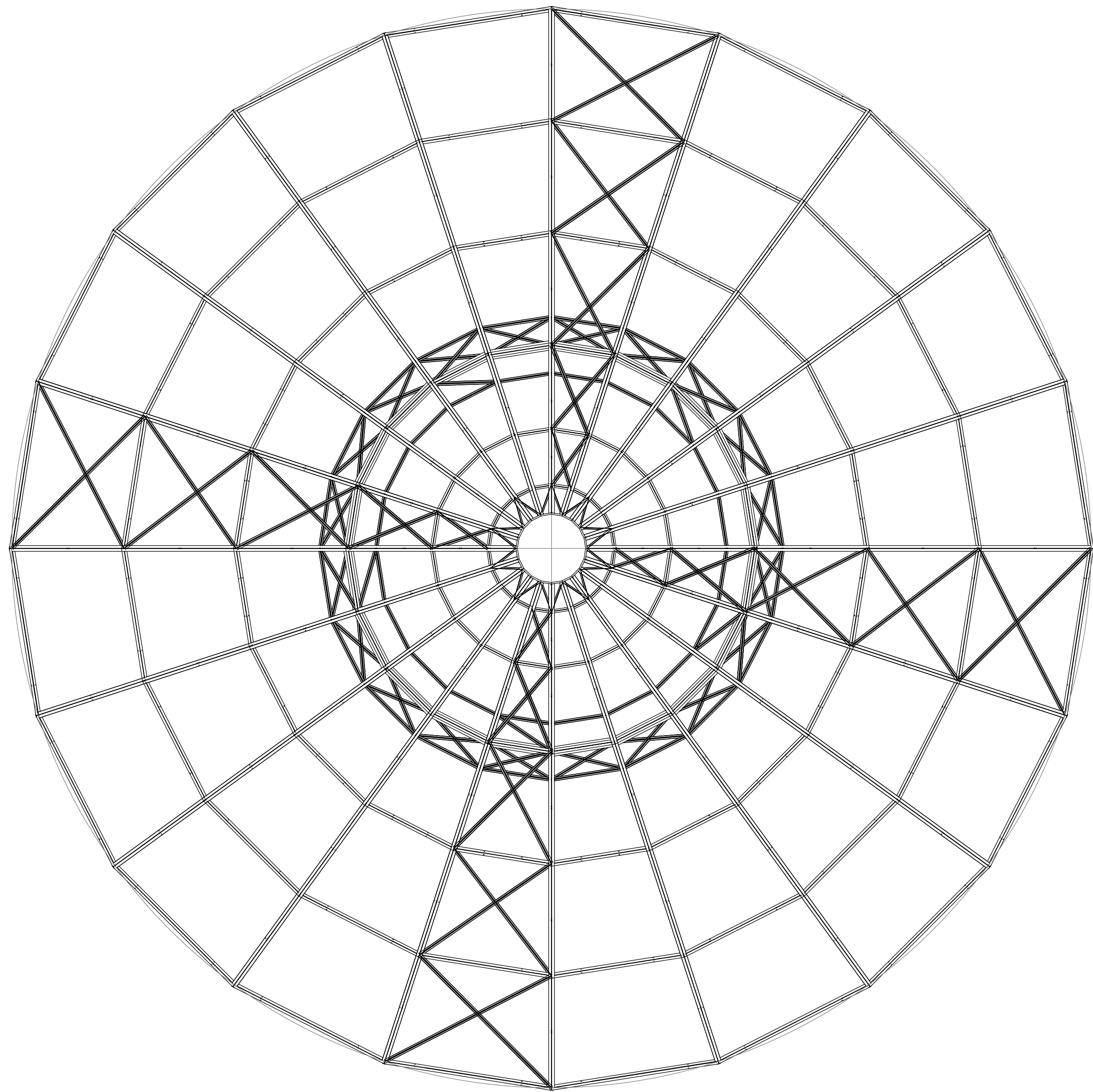
RESERVOIR ROOF STEELWORK LAYOUT SCALE 1:150
